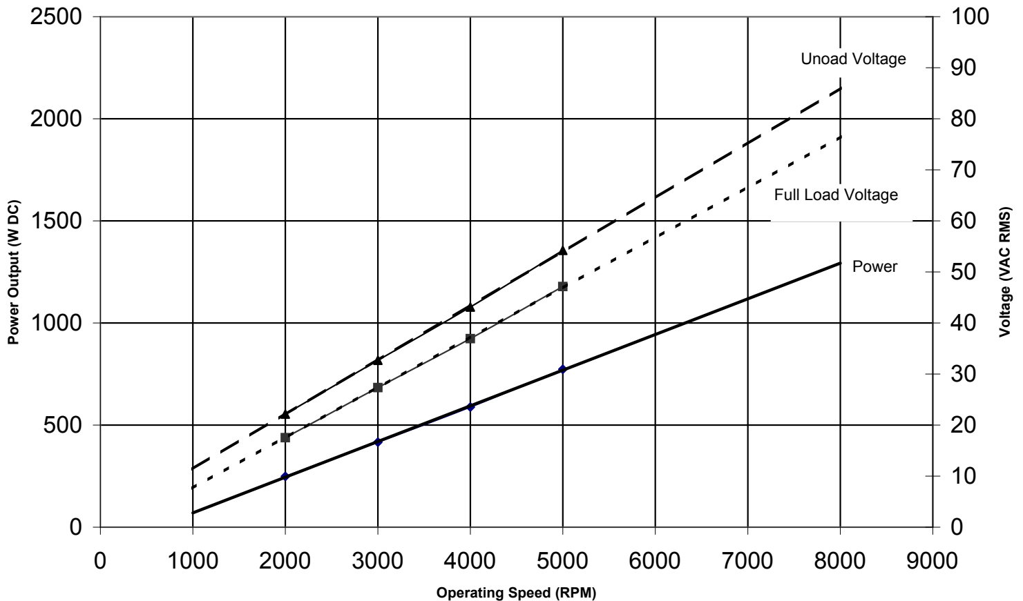
Rated Power vs RPM S676-400U-01 (120 Max °C Stator Temperature)
