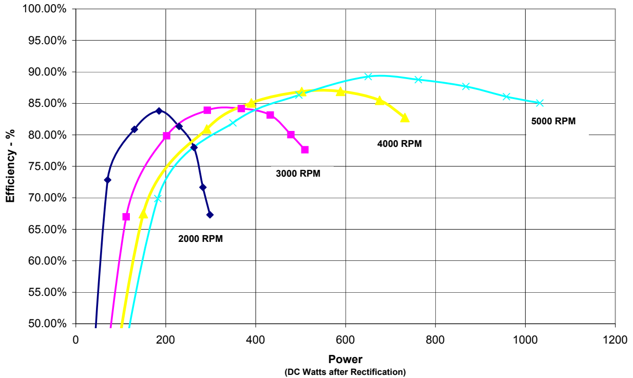
Efficiency v. Output S676-400U-01
