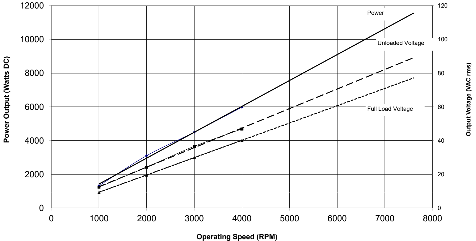
S676-800U-03 Rated Power vs RPM (120°C Max Stator Temperature)
